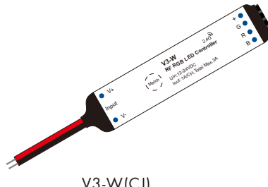
V3-W(CJ) Cable In /4P Female Jack Out Version
